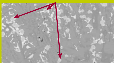
Ultra-refined complex borocarbides in 500 nm
