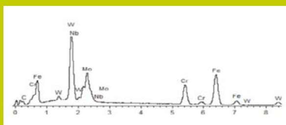
SEM / EDS spectrum showing W-Nb-Mo-rich borocarbides
