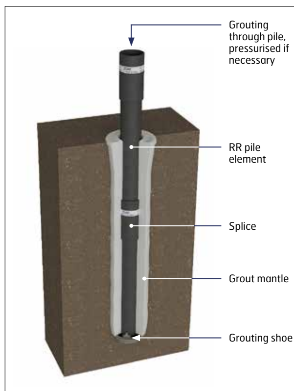
Figure 7. Grouted RR pile
