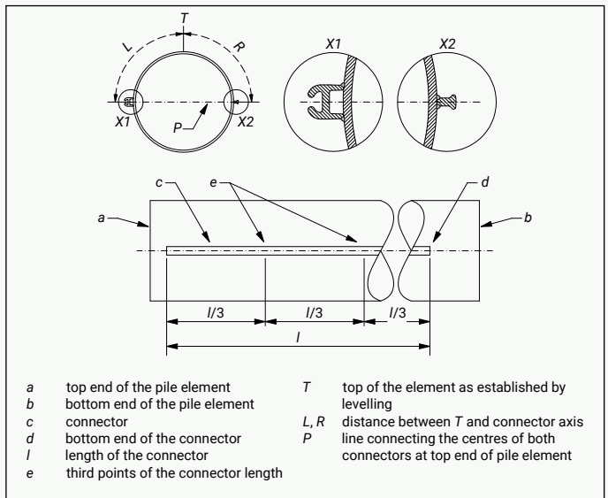
Figure 28. Positions of check points for tolerances of connectors.
