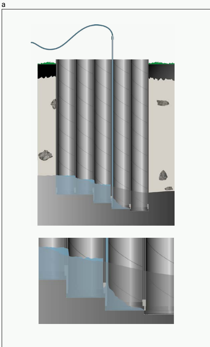
Figure 20a and 20b. Grouting behind and under an RD pile wall.
