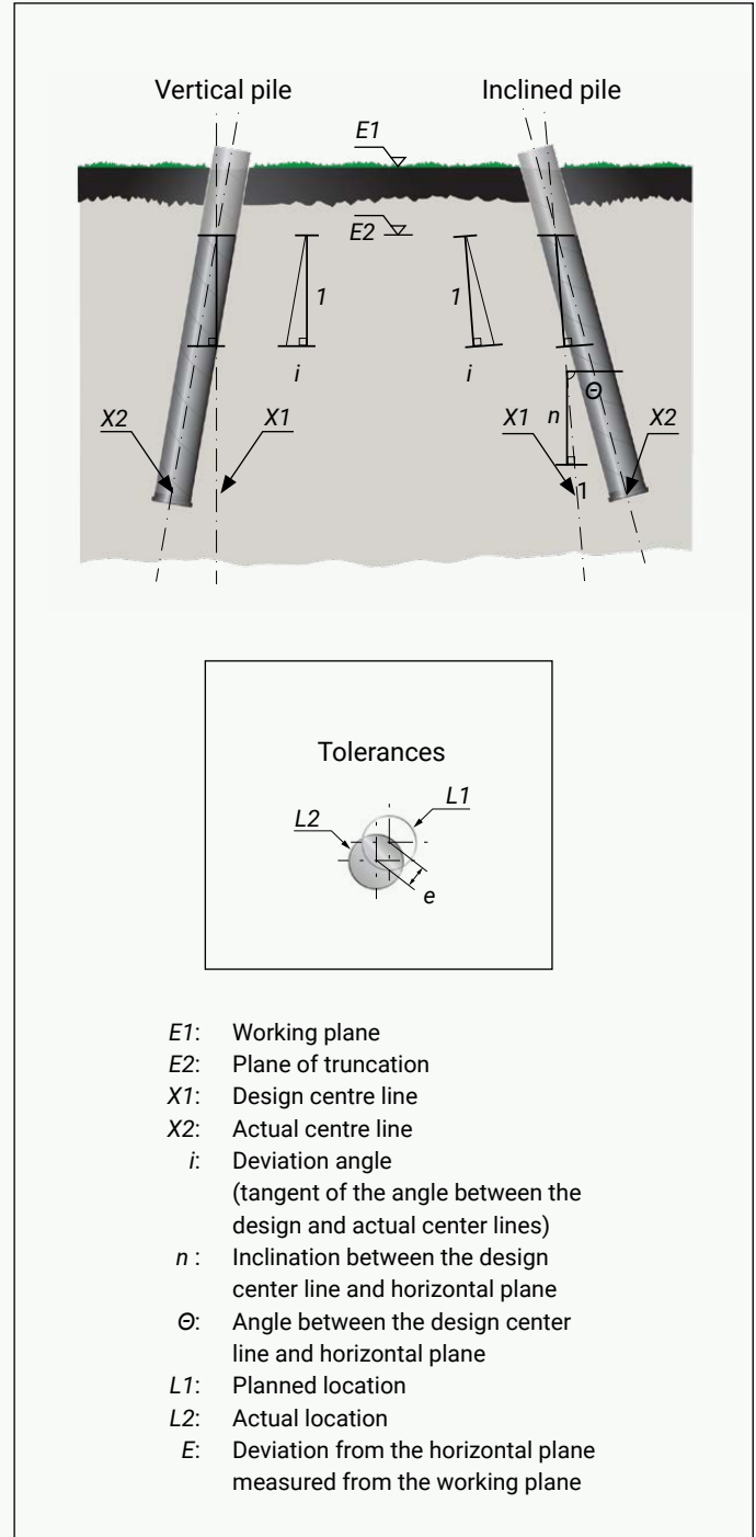
Figure 31. Definitions for geometrical tolerances in construction
