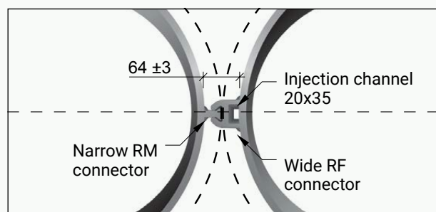
Figure 11. RM/RF connectors
