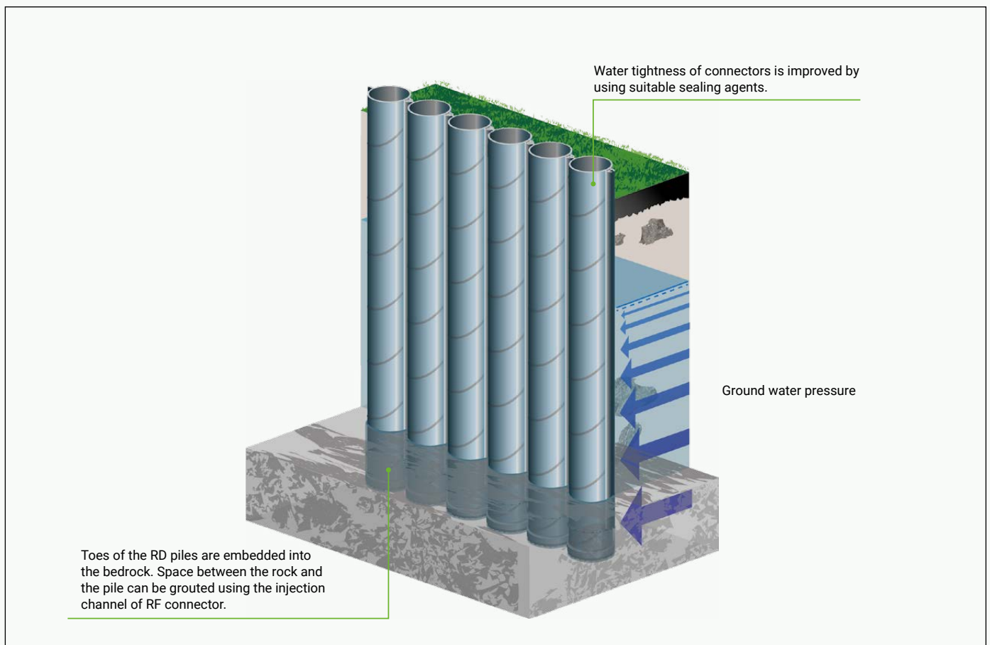
Figure 19. Watertight RD pile wall.
