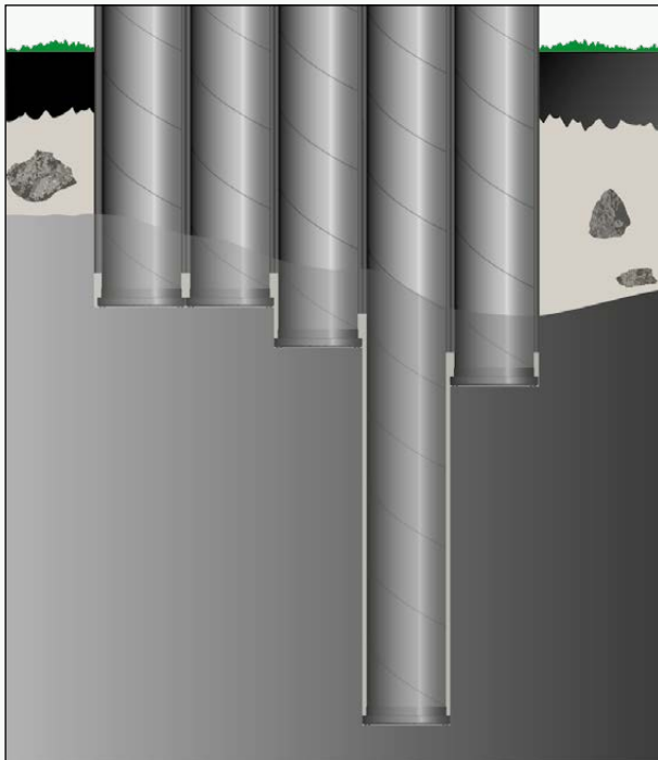
Figure 30. Ending of a connector when a pile is required to be installed at a lower level than the previous one.
