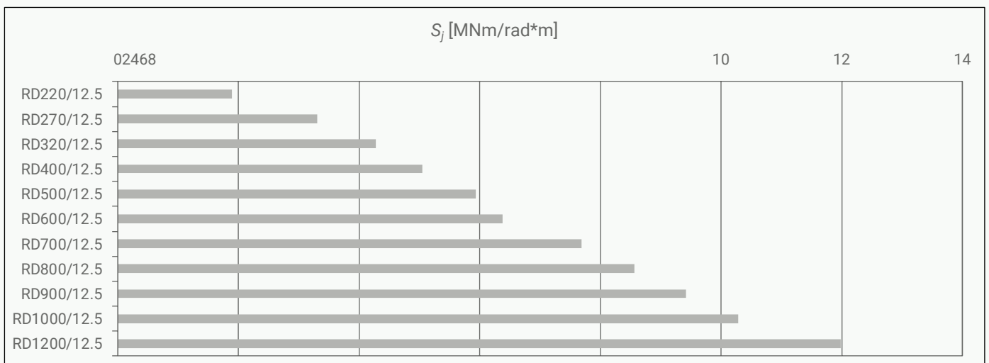
Figure 15. Stiffness of non-grouted RD pile wall. Pile sizes RD220/12.5 ... 1200/12.5, RM/RF connectors. Embedment length 3 \cdot d into integral bedrock.
