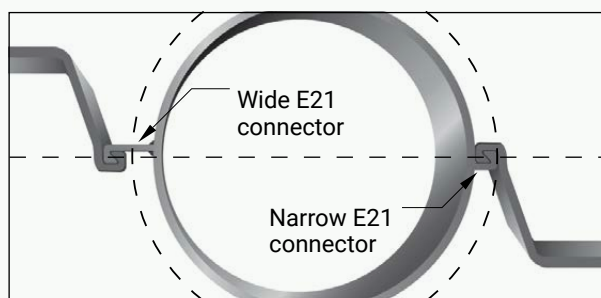
Figure 12. E21 connectors
