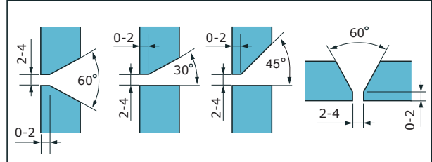
Figure 13. Types of joint preparation for welding without backing.
