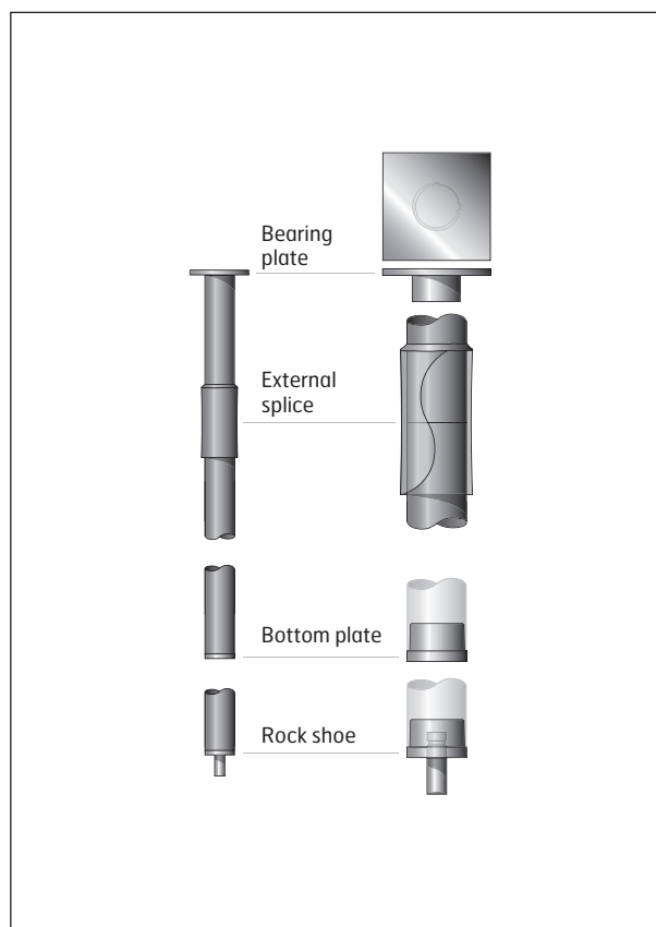
Figure 1. Structure and parts of RR piles, pile sizes RR75 to RR220.
