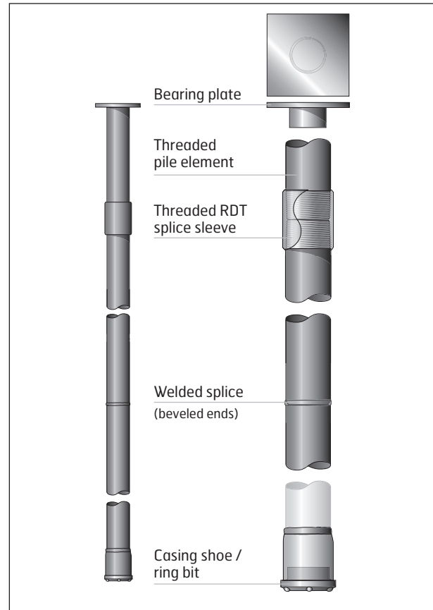
Figure 4. Structure of RD micropile.
