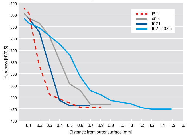
Gas nitriding of Toolox® 44
