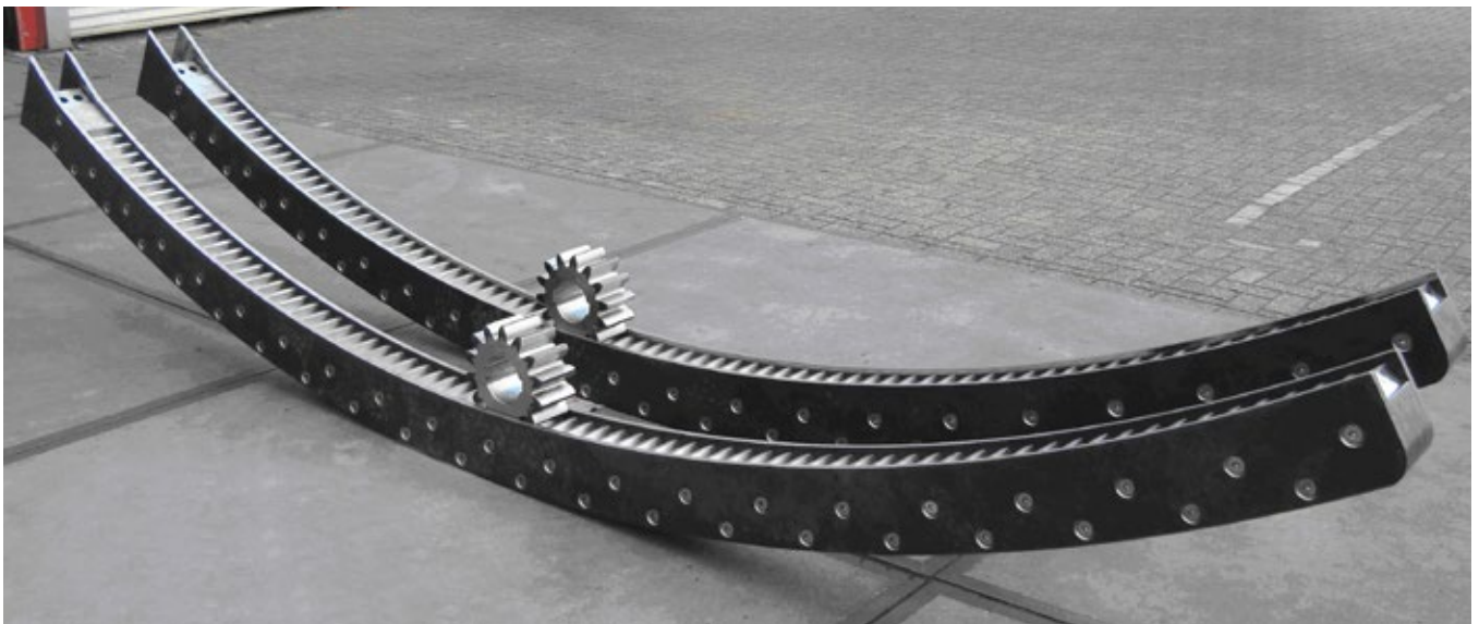
Fig. 1 Toolox® 44 gear rack for a bridge.
